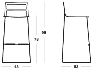
high stool L 43 P 53 H 99 H (seat) 78
