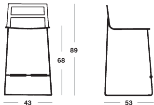
low stool L 43 P 53 H 89 H (seat) 68
